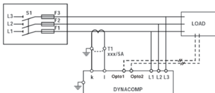
Three-phase system
